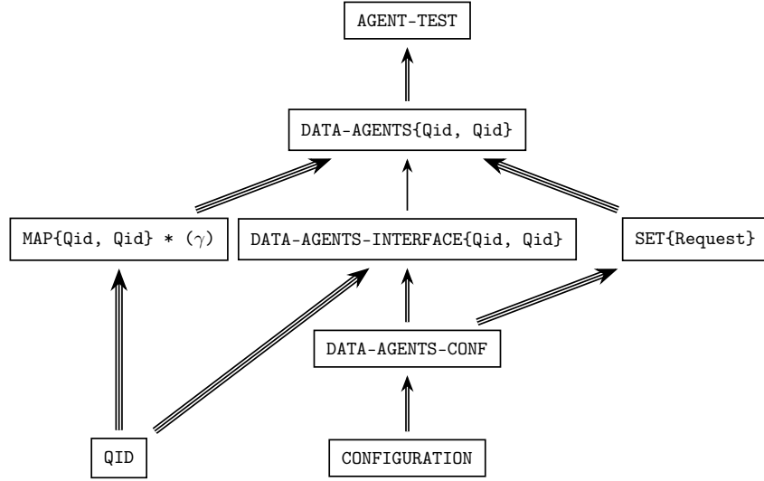
Figure 8.3: Importation graph of data-agents modules
