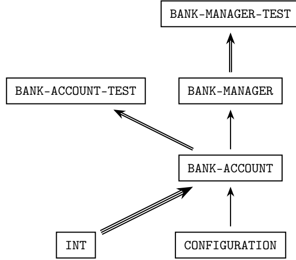
Figure 8.1: Importation graph of bank modules
