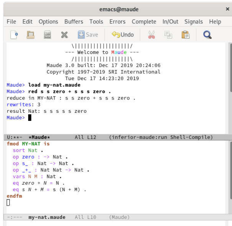
Figure 2.2: Running Maude inside Emacs
